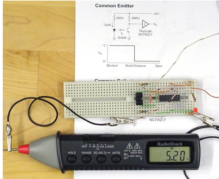
Photo - Optical Interrupter Open Fairchild H21A1
