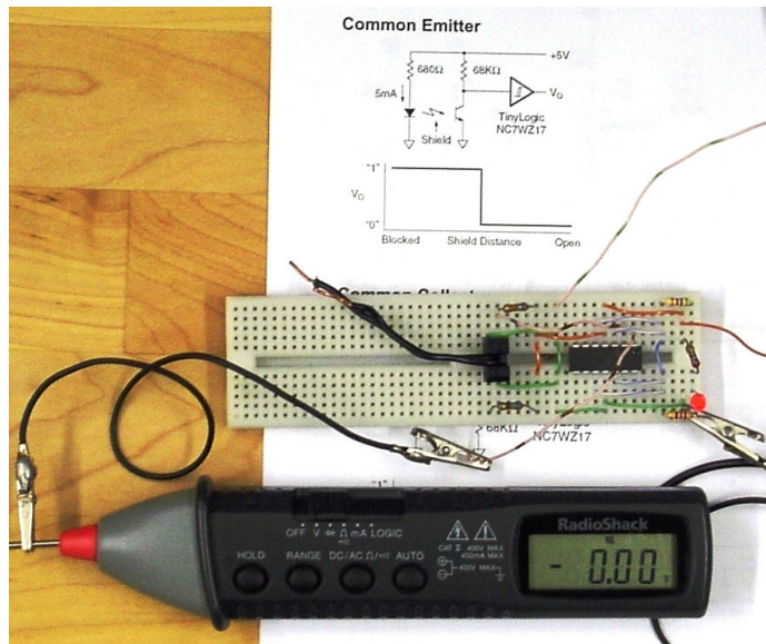
Photo - Optical Interrupter Blocked Fairchild H21A1
